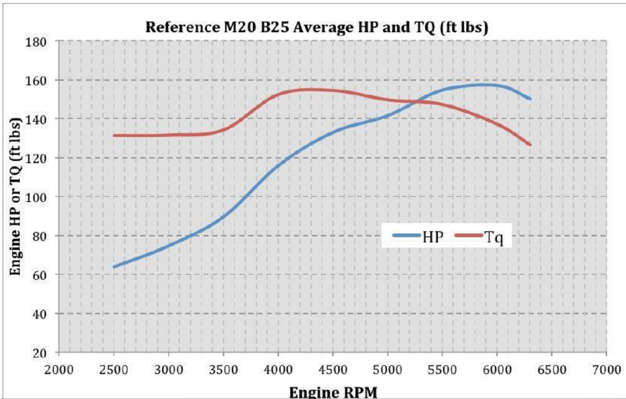
Figure 1 Dynamometer Graph M20 B25 Reference
